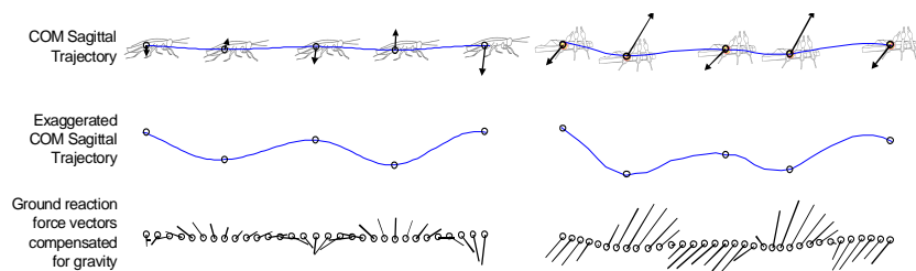
Figure 5. Ground reaction force vectors superimposed onto position data for an entire stride period. The vertical axis of the middle plot is exaggerated for detail. The ground reaction force vectors shown have been compensated for gravity by subtracting the weight of the robot from the vertical force measurement.
