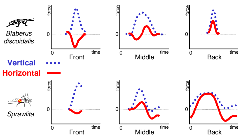
Figure 6. Plots of the individual leg ground reaction forces for Blaberus discoidalis [22] and Sprawlita . As indicated, dragging occurs in the middle and rear legs of Sprawlita during locomotion. This and the relative lack of deceleration provided by the front legs account for differences in locomotion dynamics.
